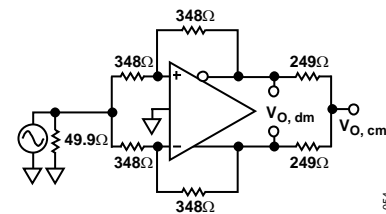
Figure 61. CMRR Test Circuit
