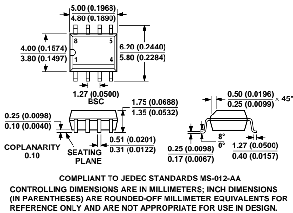
Figure 82. 8-Lead Standard Small Outline Package [SOIC] Narrow Body (R-8) Dimensions shown in millimeters and (inches)
