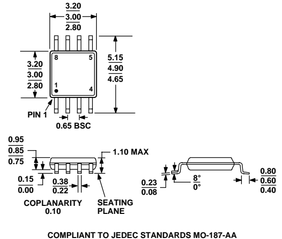
Figure 83. 8-Lead Mini Small Outline Package [MSOP] (RM-8) Dimensions shown in millimeters
