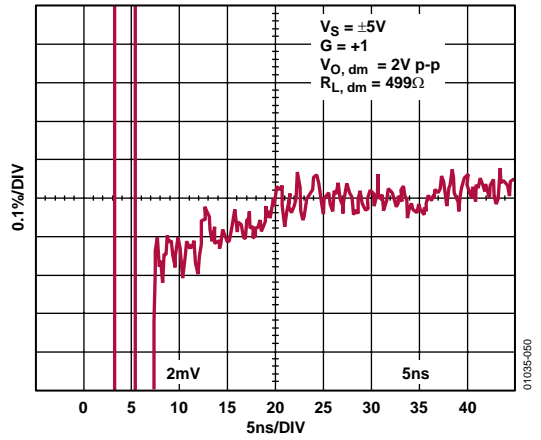
Figure 44. 0.1% Settling Time
