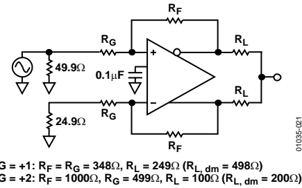
Figure 59. Test Circuit for Output Balance
